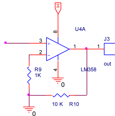
Fig. 6. Non-Inverting Amplifier Circuit
