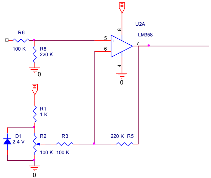
Fig. 5. Differensial Amplifier Circuit
