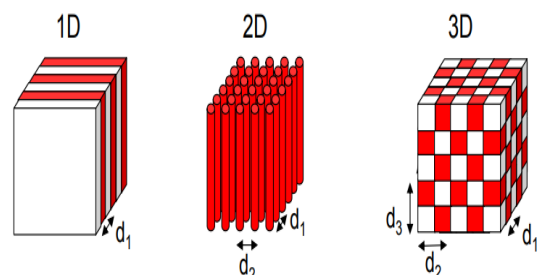
FIGURE 1. Photonic Crystals [1]
